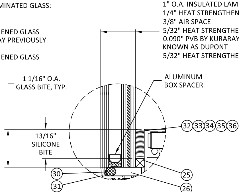
GLAZING DETAIL 4
