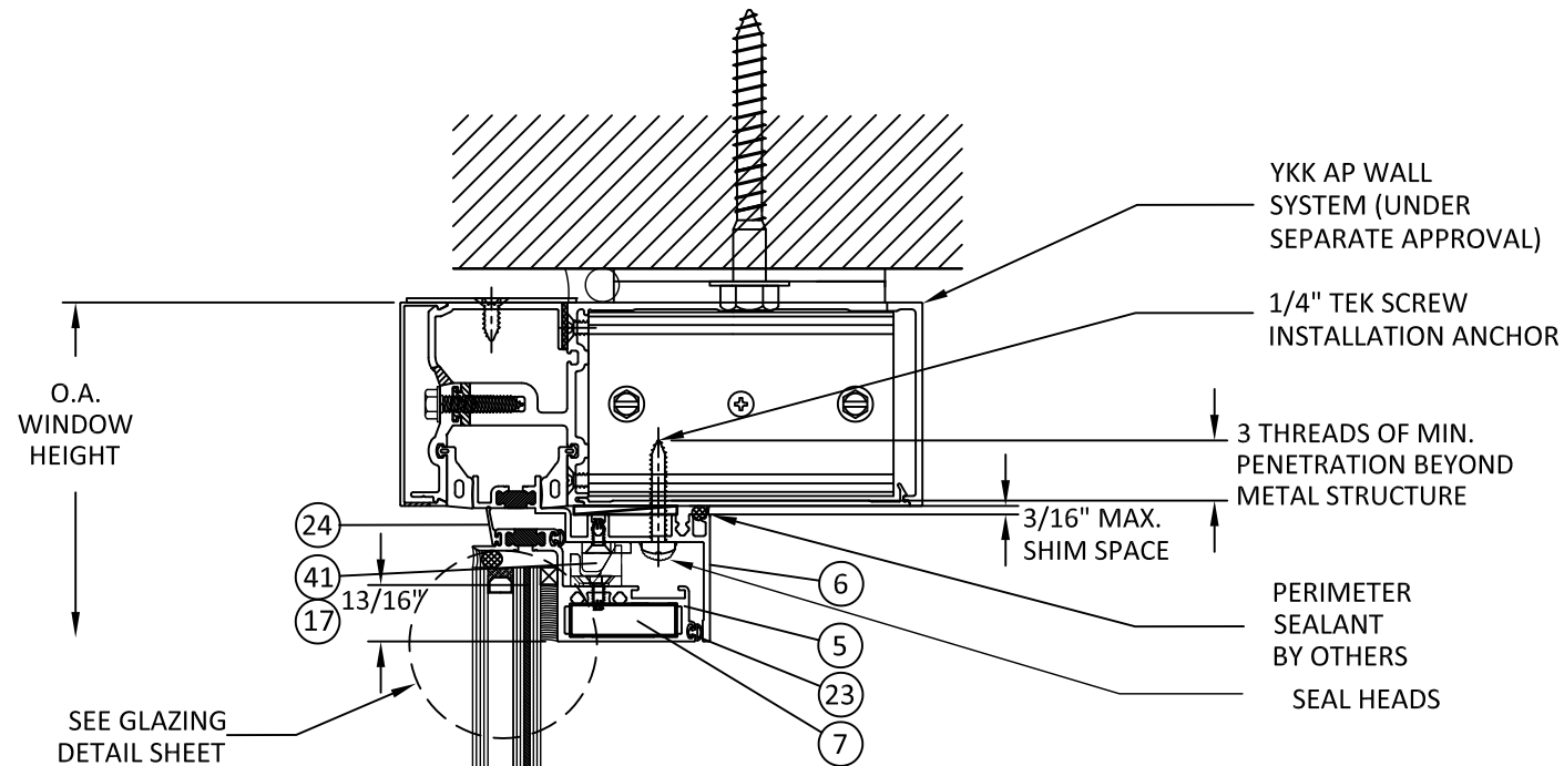
I 6 VERTICAL SECTION VENT HEAD - YKK AP WALL SYSTEM POCKET FRAME
