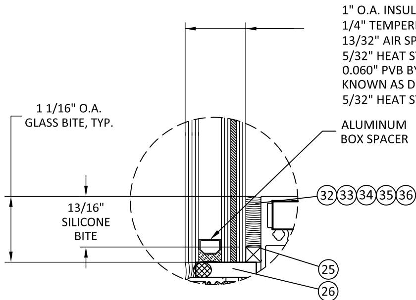
GLAZING DETAIL 2
