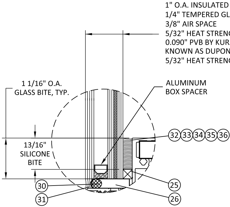
GLAZING DETAIL 1
