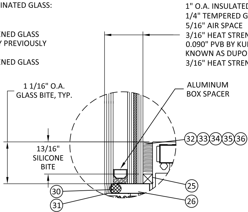
GLAZING DETAIL 3
