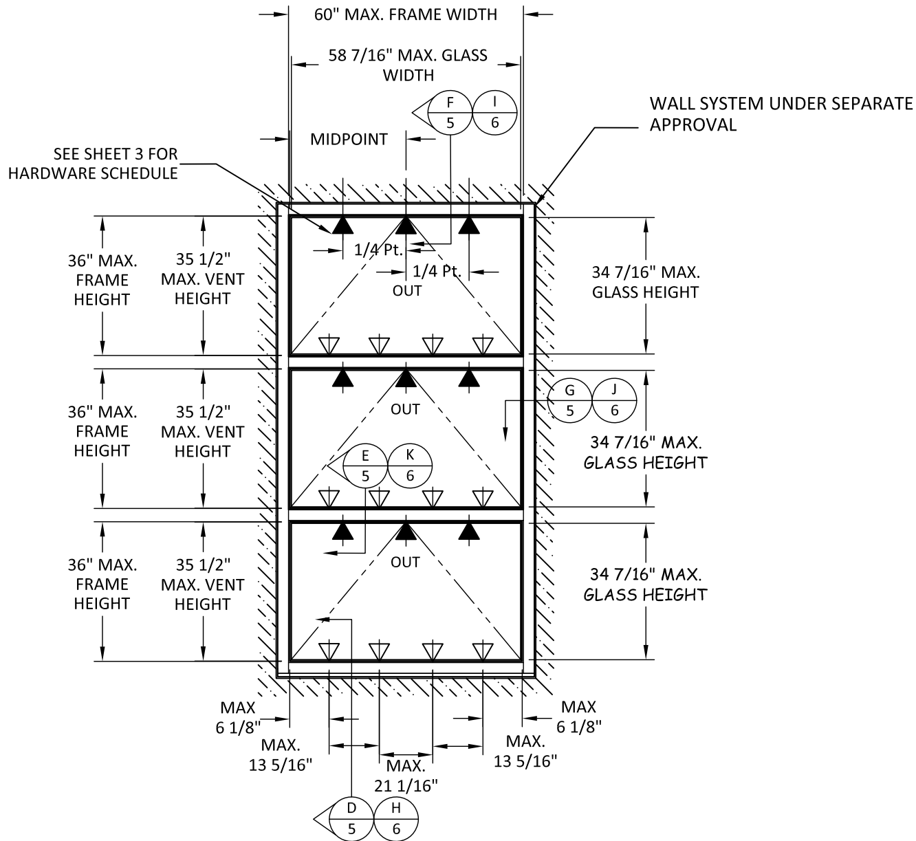
ELEVATION TYPICAL STOREFRONT/WALL
