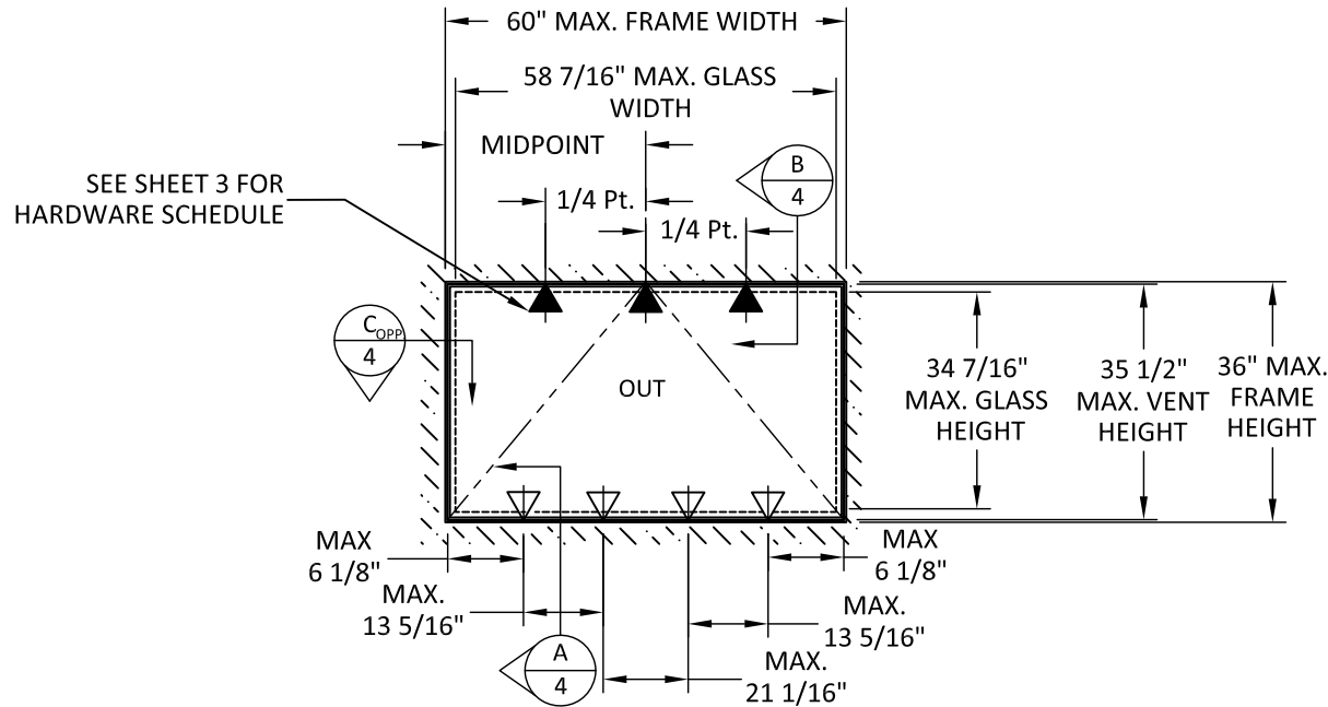
ELEVATION MULTI-POINT LOCK
