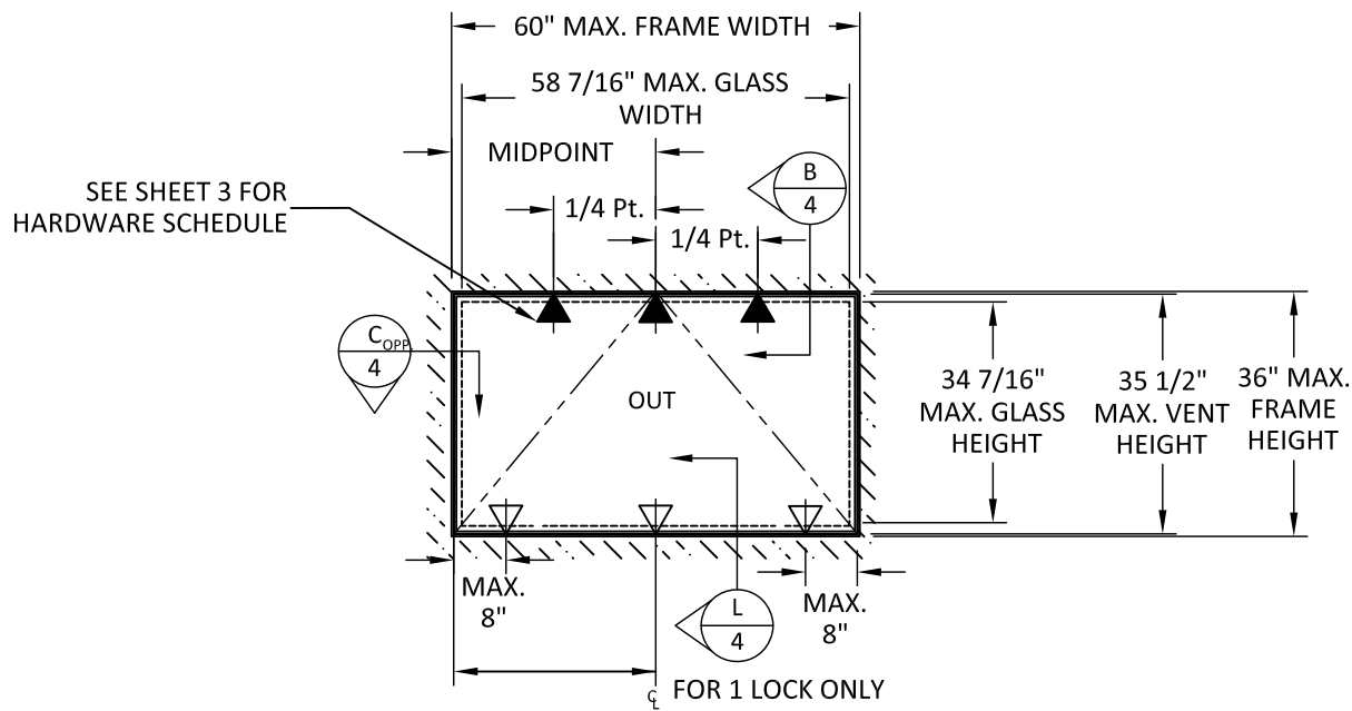
ELEVATION CAM LOCK
